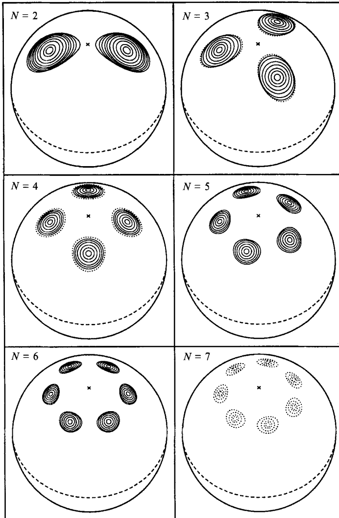
FIGURE 12. Finite-area multiple-vortex equilibria for \vartheta_0 = 60^\circ . This is an orthographic projection from 65^\circ latitude and 90^\circ longitude. The cross indicates the pole, and the dashed line the equator. Solid (dotted) lines indicate stable (unstable) equilibria (cf. §3.2).
